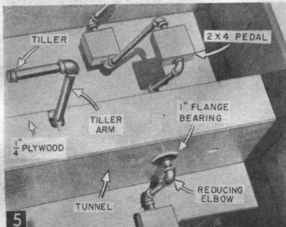
Welded pipe pedal units ride in reamed pipe flange bearings mounted on each side of the chain tunnel.
