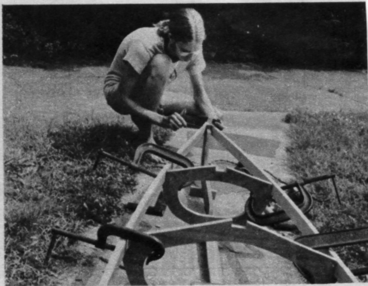
HOLD shear clamps and keelson to frame members with C clamps for screwing, gluing.
