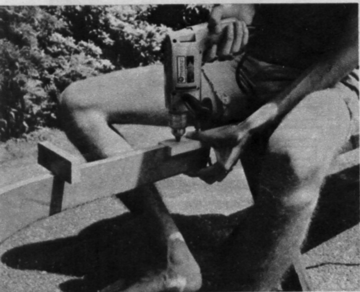
FASTEN keelson (nominally a 1x2) to stem and stern pieces with glue and brass screws.
