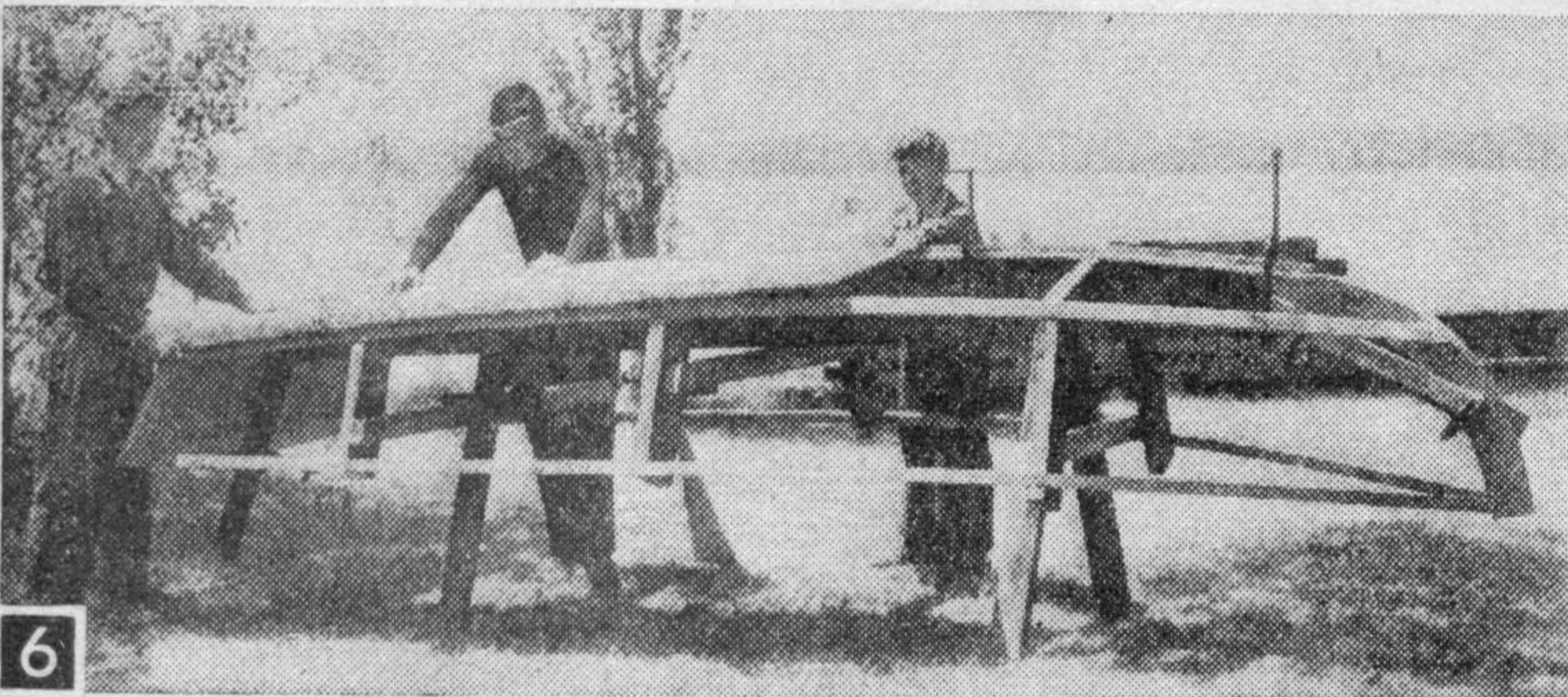
6 Covering the frame with plywood.
