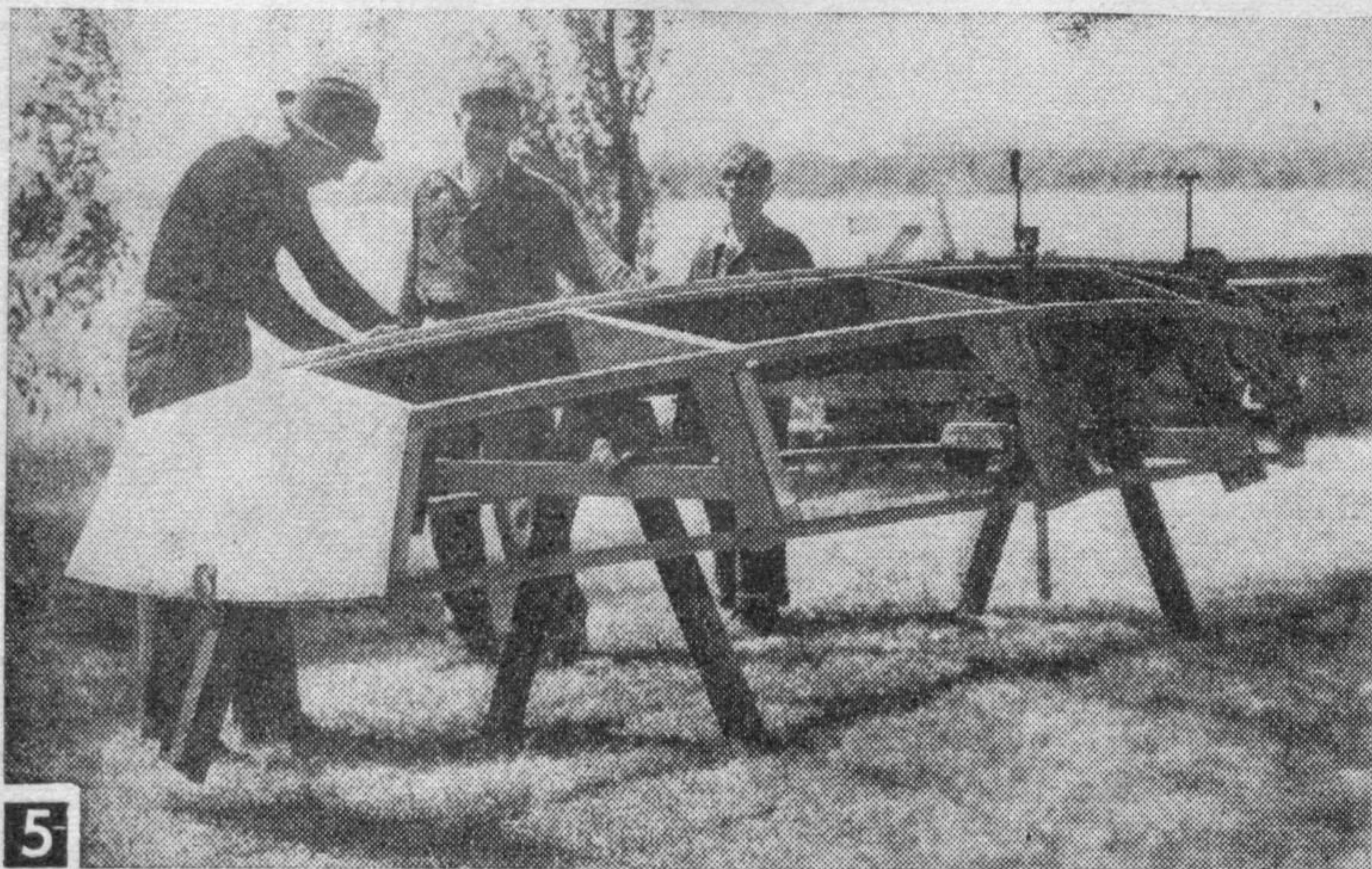
5 The completed framework.
