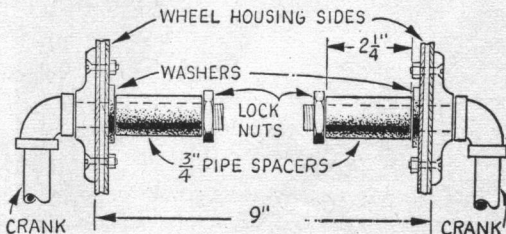
CRANK ARRANGEMENT WHEN MOTOR IS USED INSTEAD OF PADDLE WHEEL
