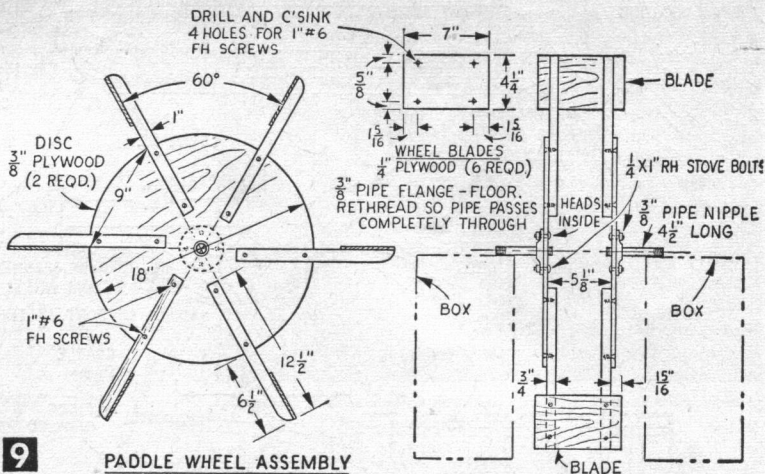
PADDLE WHEEL ASSEMBLY
