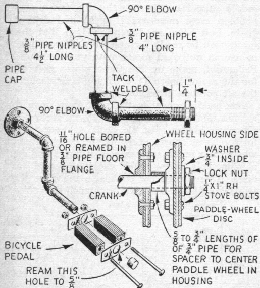
PADDLE-WHEEL CRANKS (2 REQD.)
