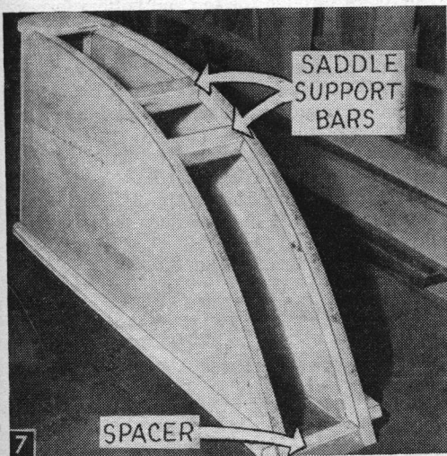
7 Paddle-wheel housing showing saddle support bars and aft spacer.
